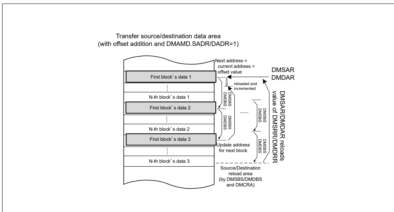
Figure 15.17 Address update in offset addition with DMAMD.SADR and DMAMD.DADR = 1
