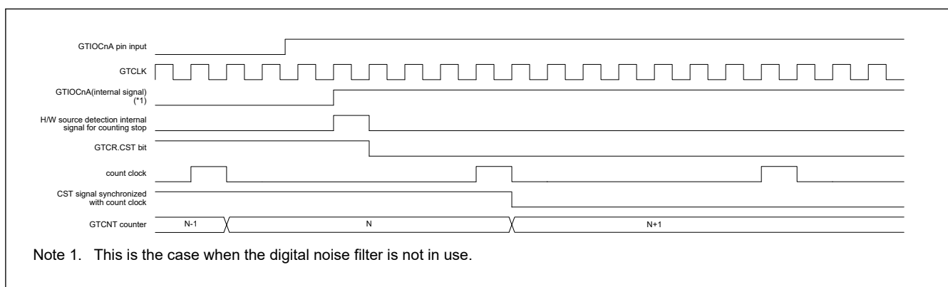
Figure 21.93 Example of Timing of Operations to Stop Counting in Response to a Rising Edge of the Input on the GTIOCN Pin
