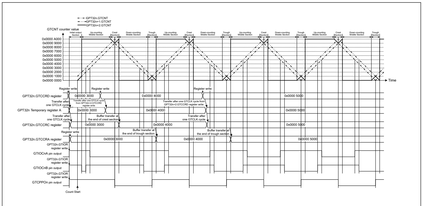
Figure 21.50 Example of Complementary PWM Mode 2 Operation (GTIOCRnA pin = High / GTIOCRnB pin = High as initial output, GTIOCRnA pin = Low / GTIOCRnB pin = High at GTCCR register compare match during up-counting, GTIOCRnA pin = High / GTIOCRnB pin = Low at GTCCR register compare match during down-counting, the dead time value is 0x0000 1000 and updating GTCCR register in middle section) (n = 4, 7)
