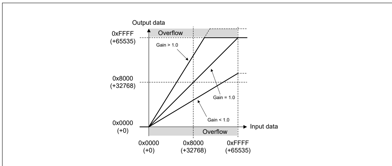
Figure 36.23 User's Gain Adjustment (16-bit data length format)
