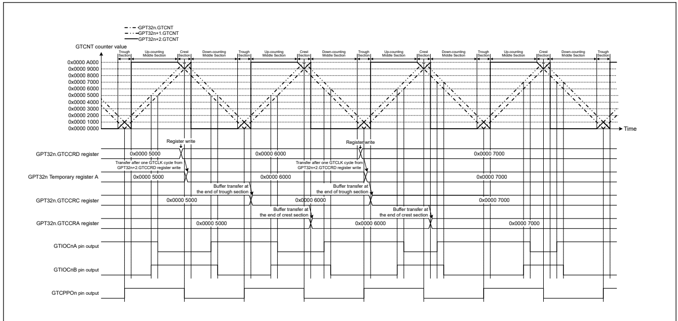
Figure 21.49 Example of Complementary PWM Mode 1 Operation (GTIOCRnA pin = Low / GTIOCRnB pin = High at GTCCR register compare match during up-counting, GTIOCRnA pin = High / GTIOCRnB pin = Low at GTCCR register compare match during down-counting, the dead time value is 0x0000 1000 and updating GTCCR register in crest and trough sections) (n = 4, 7)
