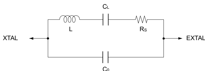
Figure 8.5 Equivalent circuit of the crystal resonator
