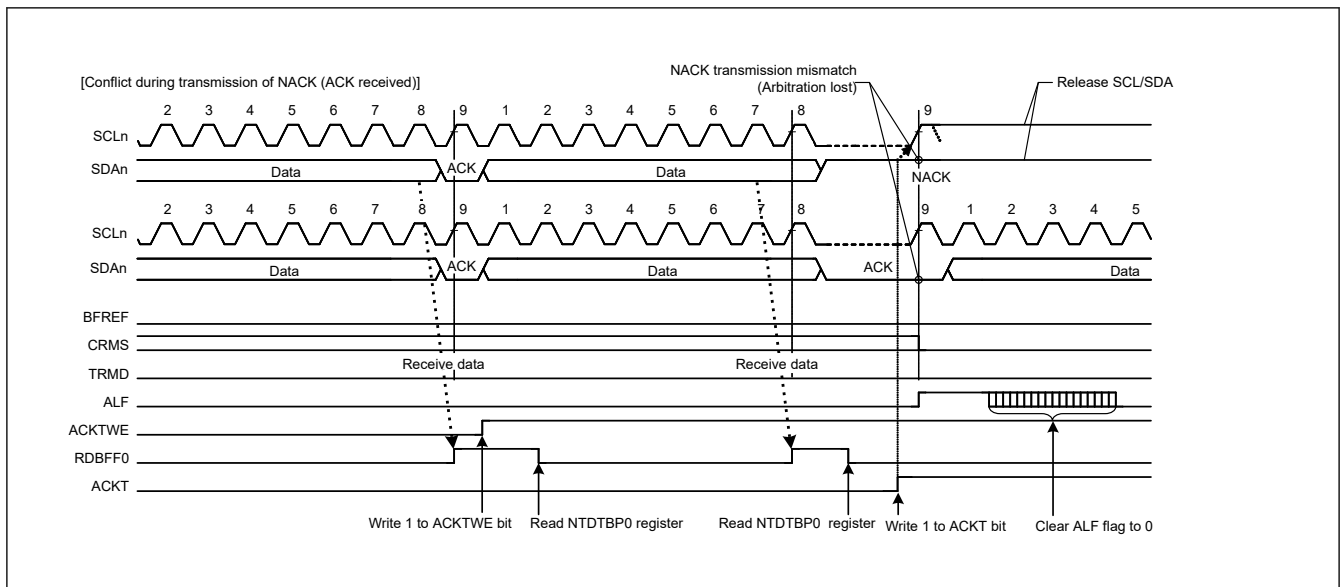
Figure 27.27 Example of arbitration-lost detection during transmission of NACK (NALE = 1)
