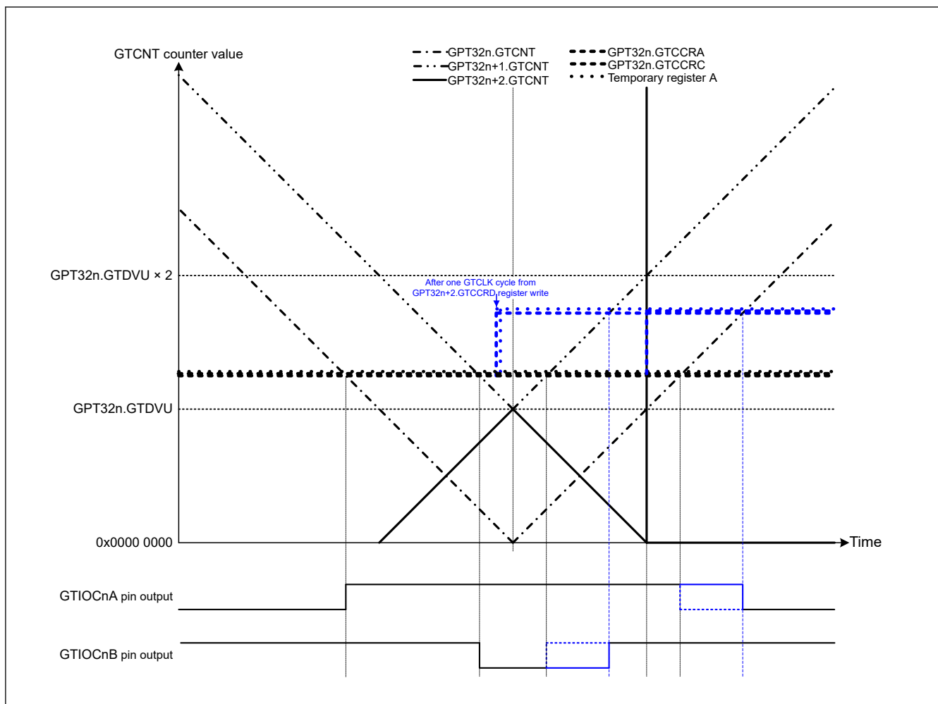
Figure 21.75 Example of Complementary PWM Mode 4 Single Buffer Operation (Down-Counting Trough Section) (Complementary PWM mode 4 single buffer operation, GTIOCN pin = Low / GTIOCNB pin = High at GTCCRA register compare match during up-counting, GTIOCN pin = High / GTIOCNB pin = Low at GTCCRA register compare match during down-counting, when a value larger than the GPT32n+2.GTCNT value is written to GTCCRD register after down-counting compare match) (n = 4, 7)
