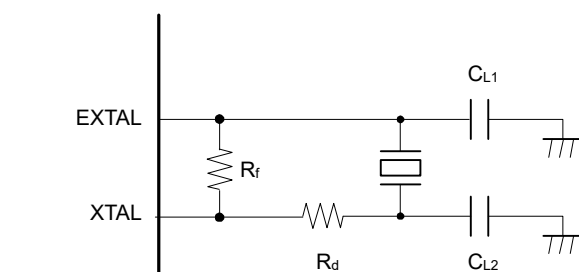
Figure 8.4 Example of crystal resonator connection
