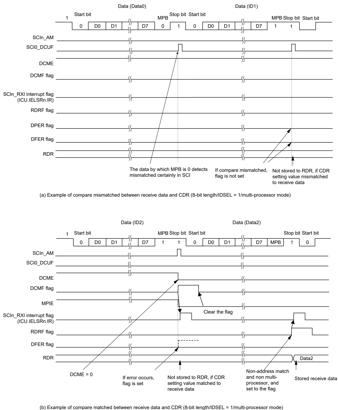
Figure 25.6 Example of address match (2) multi-processor mode
