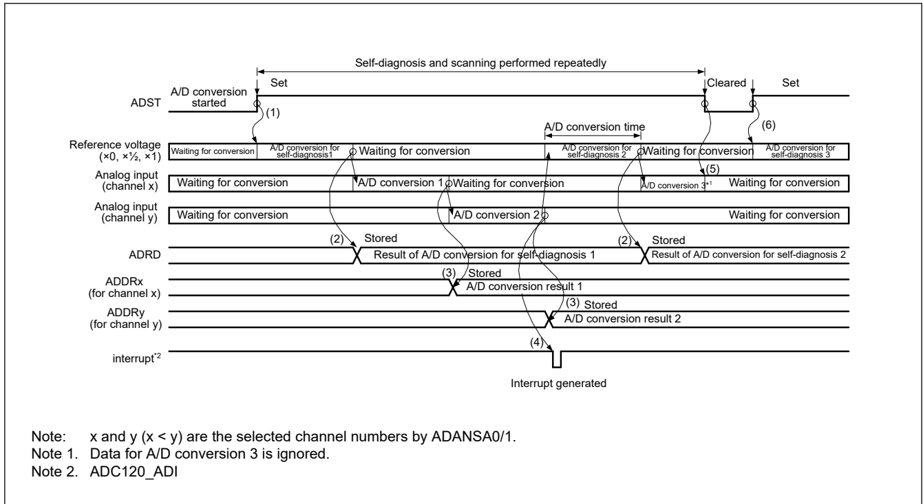
Figure 30.13 Example basic operation in continuous scan mode when the analog inputs (channel x and y) selected with self-diagnosis
