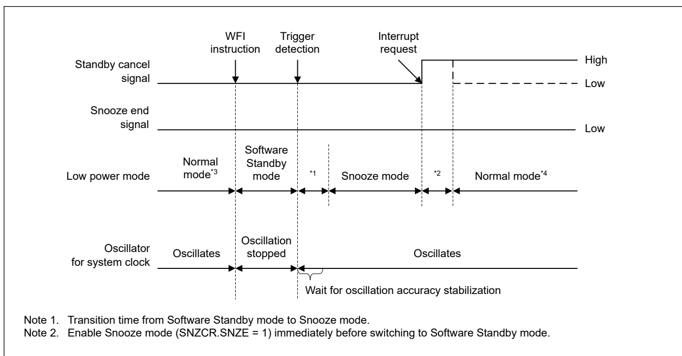
Figure 10.11 Canceling of Snooze mode when an interrupt request signal is not generated
