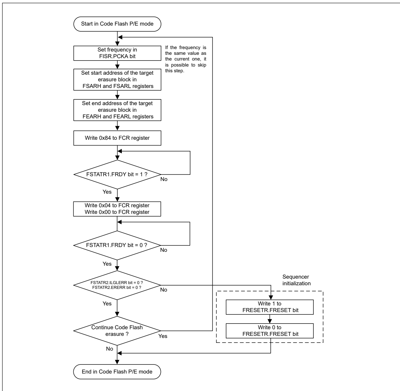
Figure 37.22 Flowchart for the code flash block erase procedure
