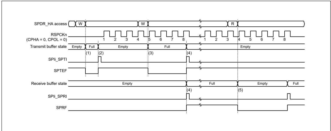
Figure 28.26 Operation example of the SPli_SPTI and SPli_SPRI interrupts when CPHA = 0 and CPOL = 0 in master mode
