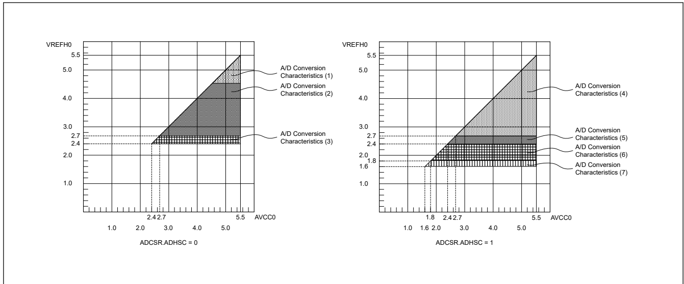
Figure 41.37 VCC to VREFH0 voltage range
